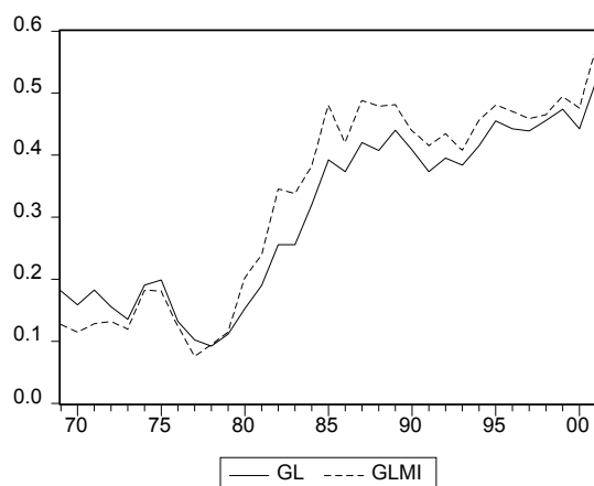
Figure 2 Plot of the Average GL Index for all 3-digit Sectors and the Average GL index for Manufacturing Industries
