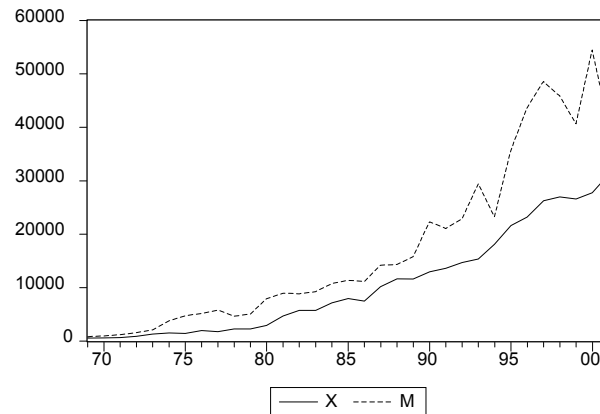
Figure 1b Plot of Manufacturing Industry Exports (XMI) and Imports (MMI)
