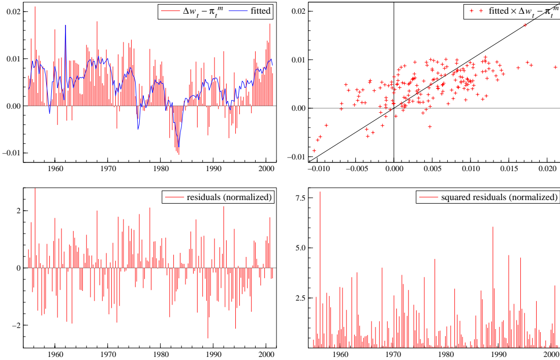
Figure 5 Nominal Wage Phillips Curve.
